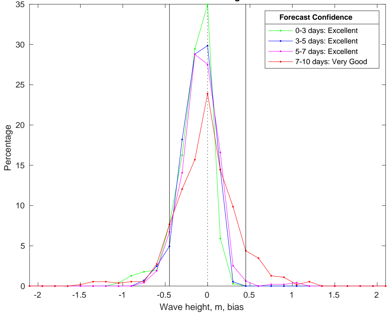
NDBC 42035 vs CMEMS Waves Bias Histogram: 08-Feb-2025
