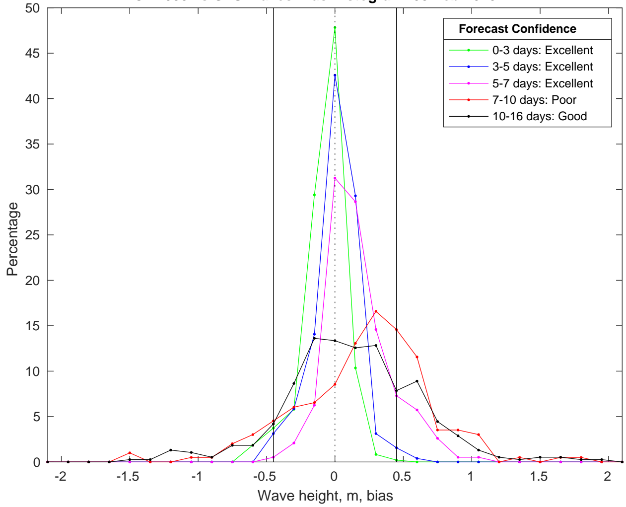
NDBC 42035 vs GFS Waves Bias Histogram: 08-Feb-2025
