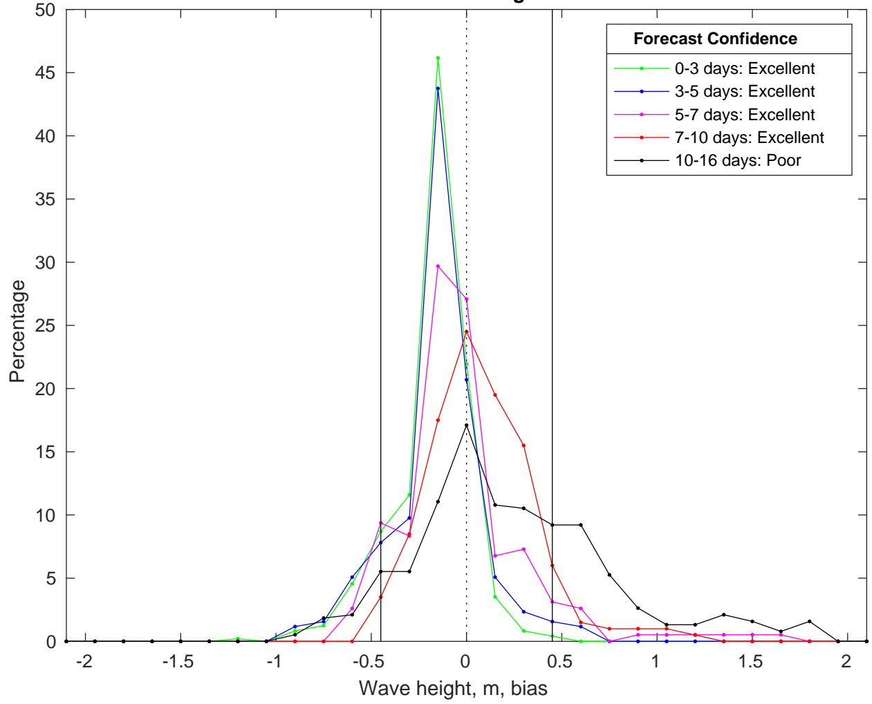
NDBC 42036 vs GFS Waves Bias Histogram: 08-Feb-2025
