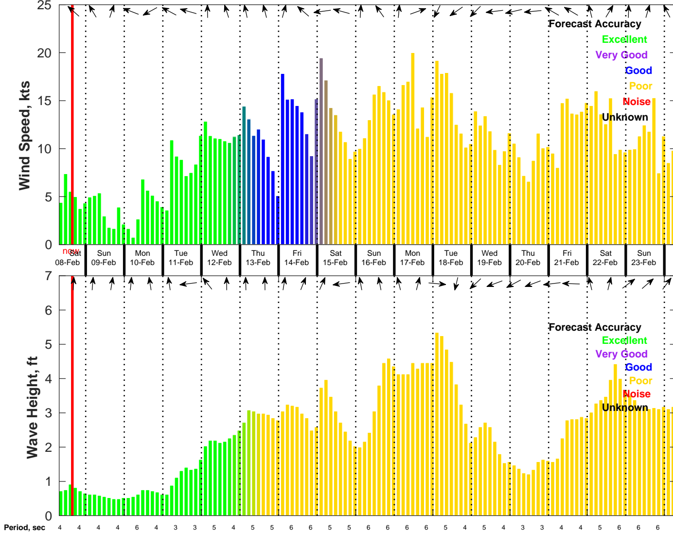
Wind & Wave Forecast for NDBC 42036 from 08-Feb-2025 07:00:00 to 24-Feb-2025 07:00:00
