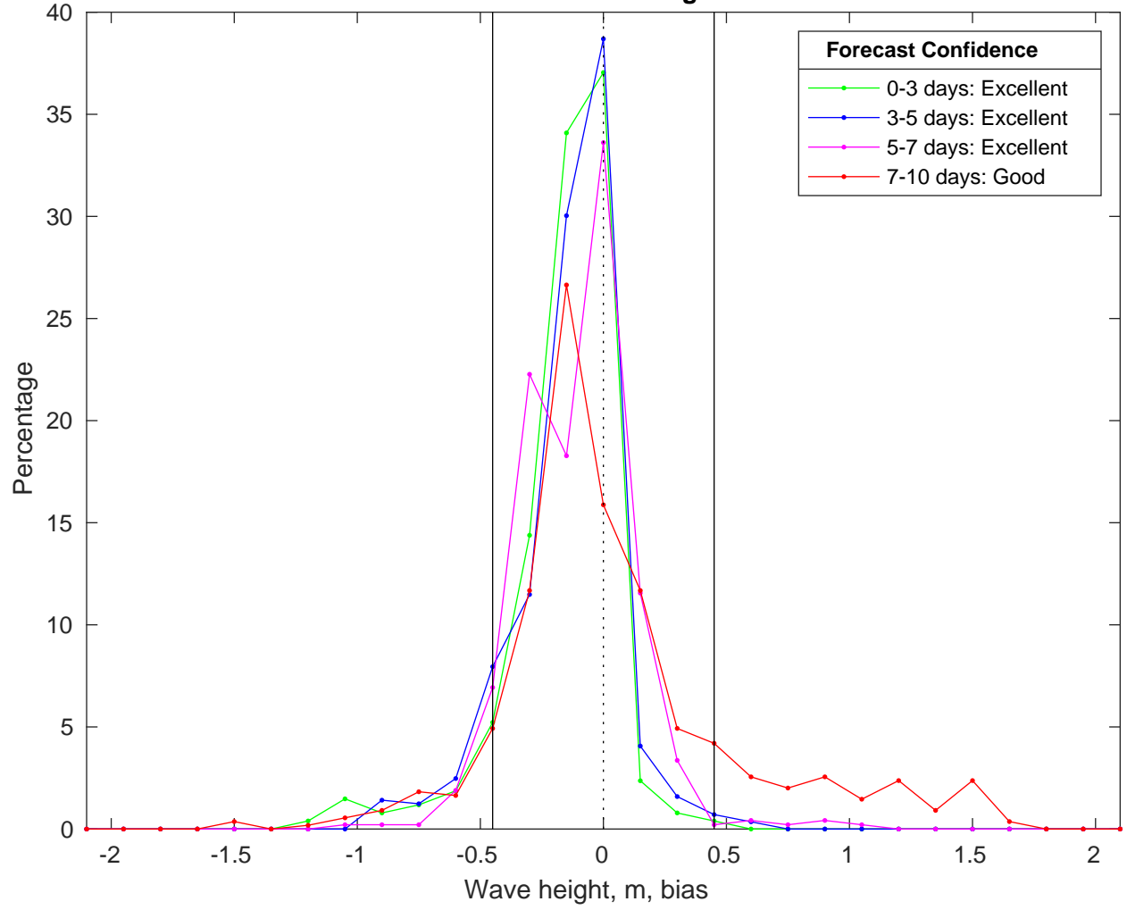
NDBC 42040 vs CMEMS Waves Bias Histogram: 08-Feb-2025
