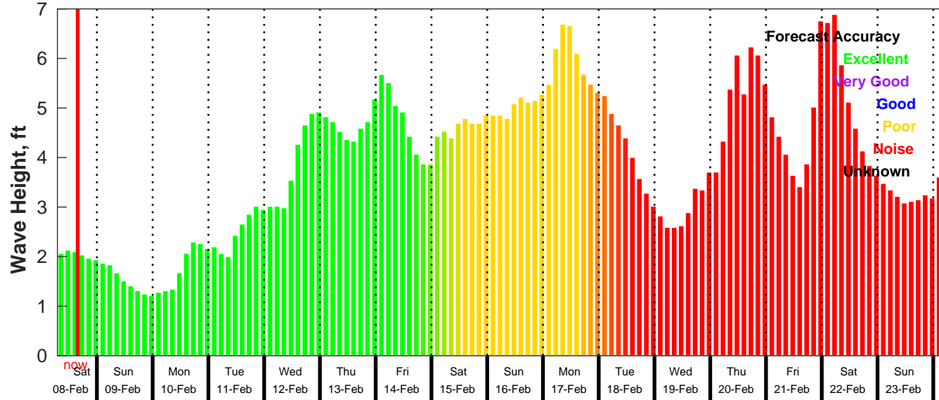
GFS Wave Forecast for NDBC 42040 from 08-Feb-2025 07:00:00 to 24-Feb-2025 07:00:00
