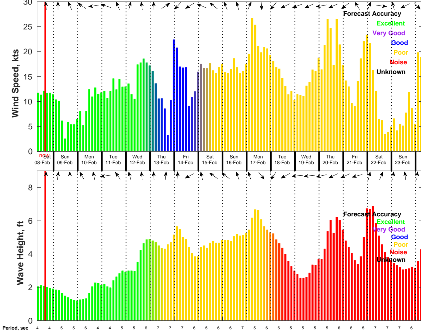
Wind & Wave Forecast for NDBC 42040 from 08-Feb-2025 07:00:00 to 24-Feb-2025 07:00:00
