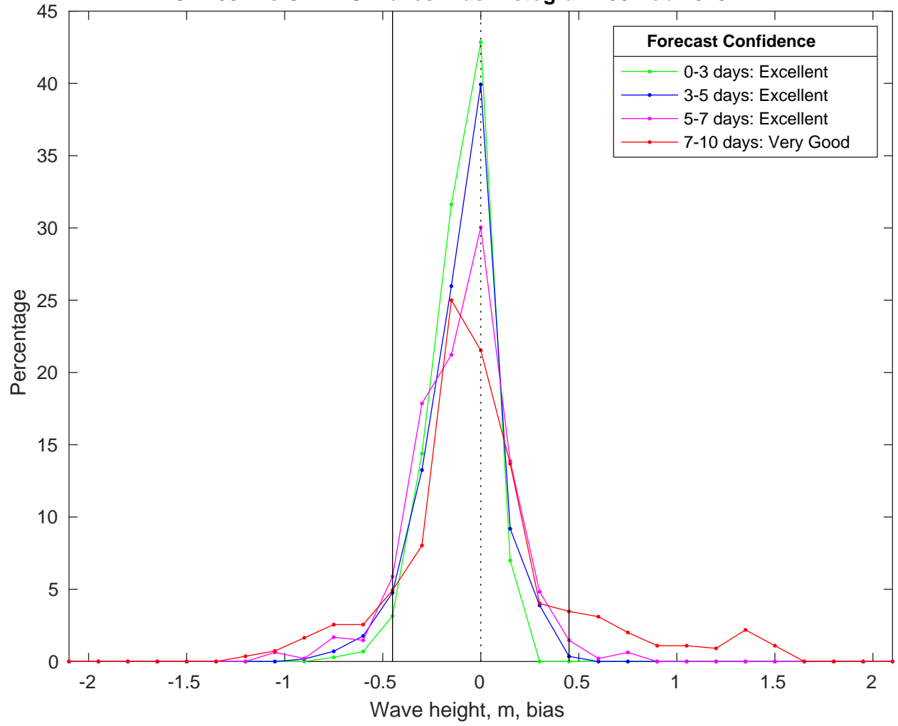
NDBC 42084 vs CMEMS Waves Bias Histogram: 08-Feb-2025
