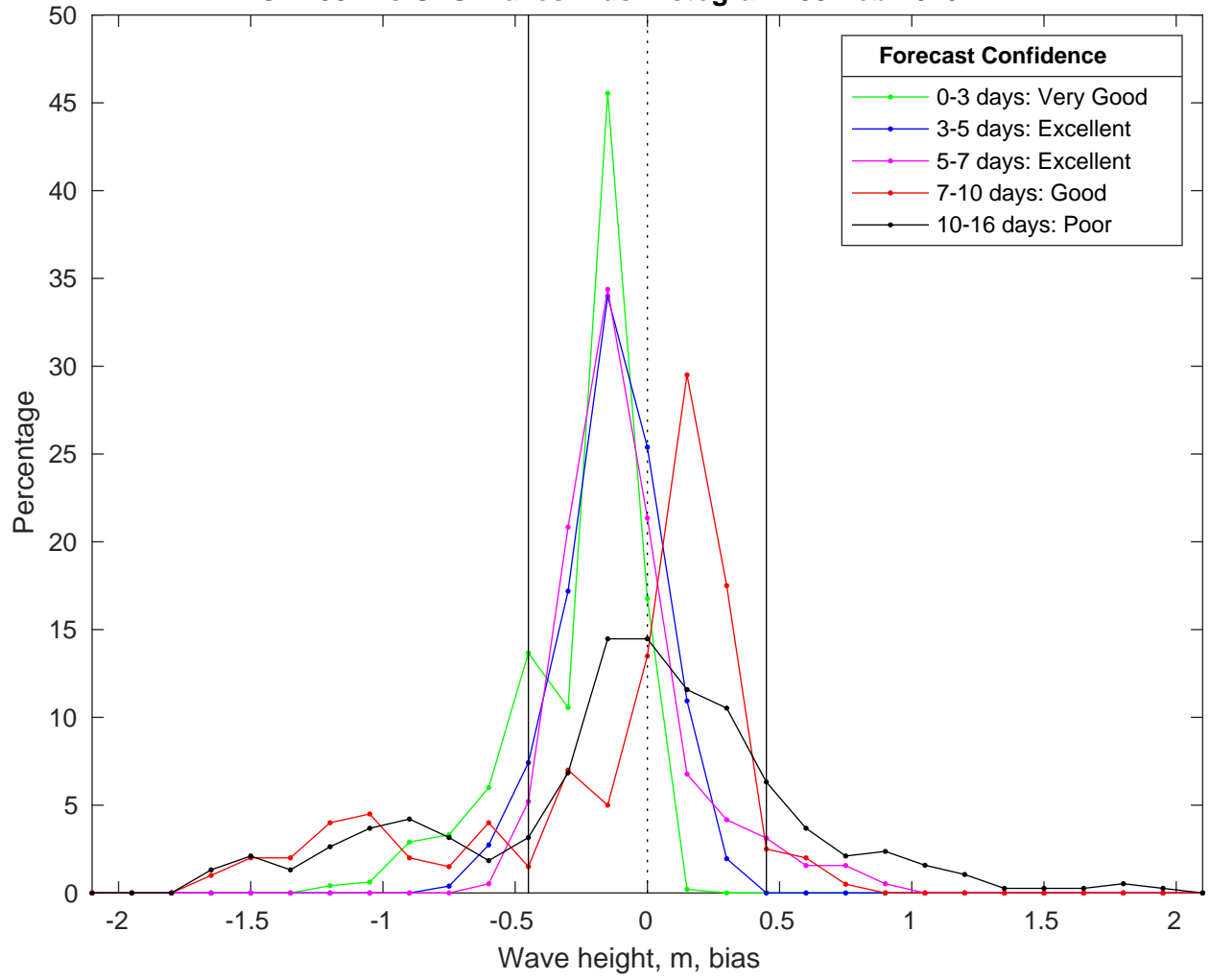
NDBC 42084 vs GFS Waves Bias Histogram: 08-Feb-2025
