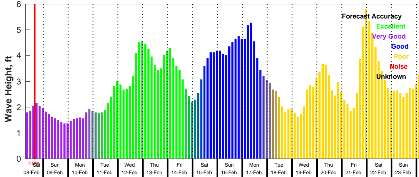
GFS Wave Forecast for NDBC 42084 from 08-Feb-2025 07:00:00 to 24-Feb-2025 07:00:00
