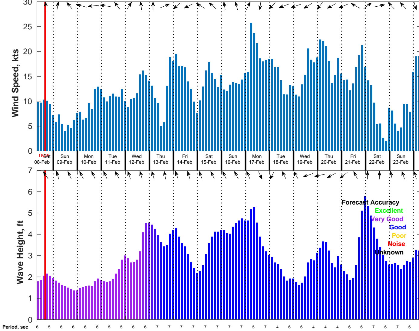
Wind & Wave Forecast for NDBC 42084 from 08-Feb-2025 07:00:00 to 24-Feb-2025 07:00:00
