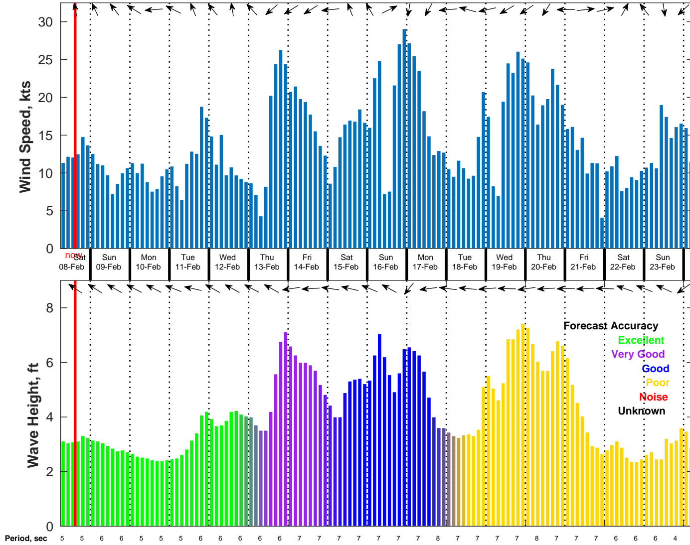
Wind & Wave Forecast for NDBC 42092 from 08-Feb-2025 06:00:00 to 24-Feb-2025 06:00:00
