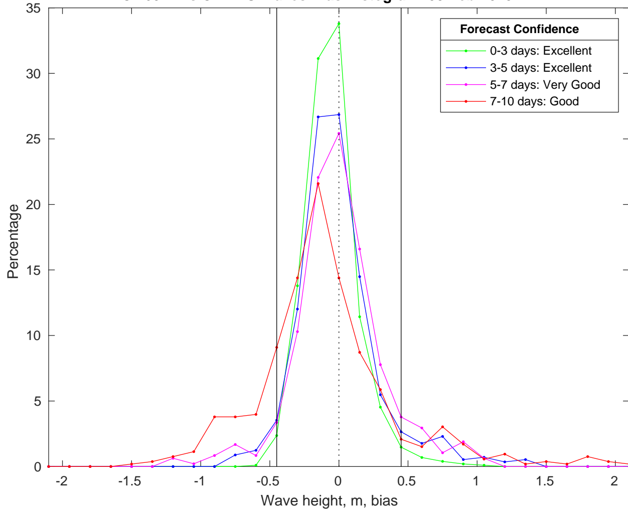
NDBC 46011 vs CMEMS Waves Bias Histogram: 08-Feb-2025
