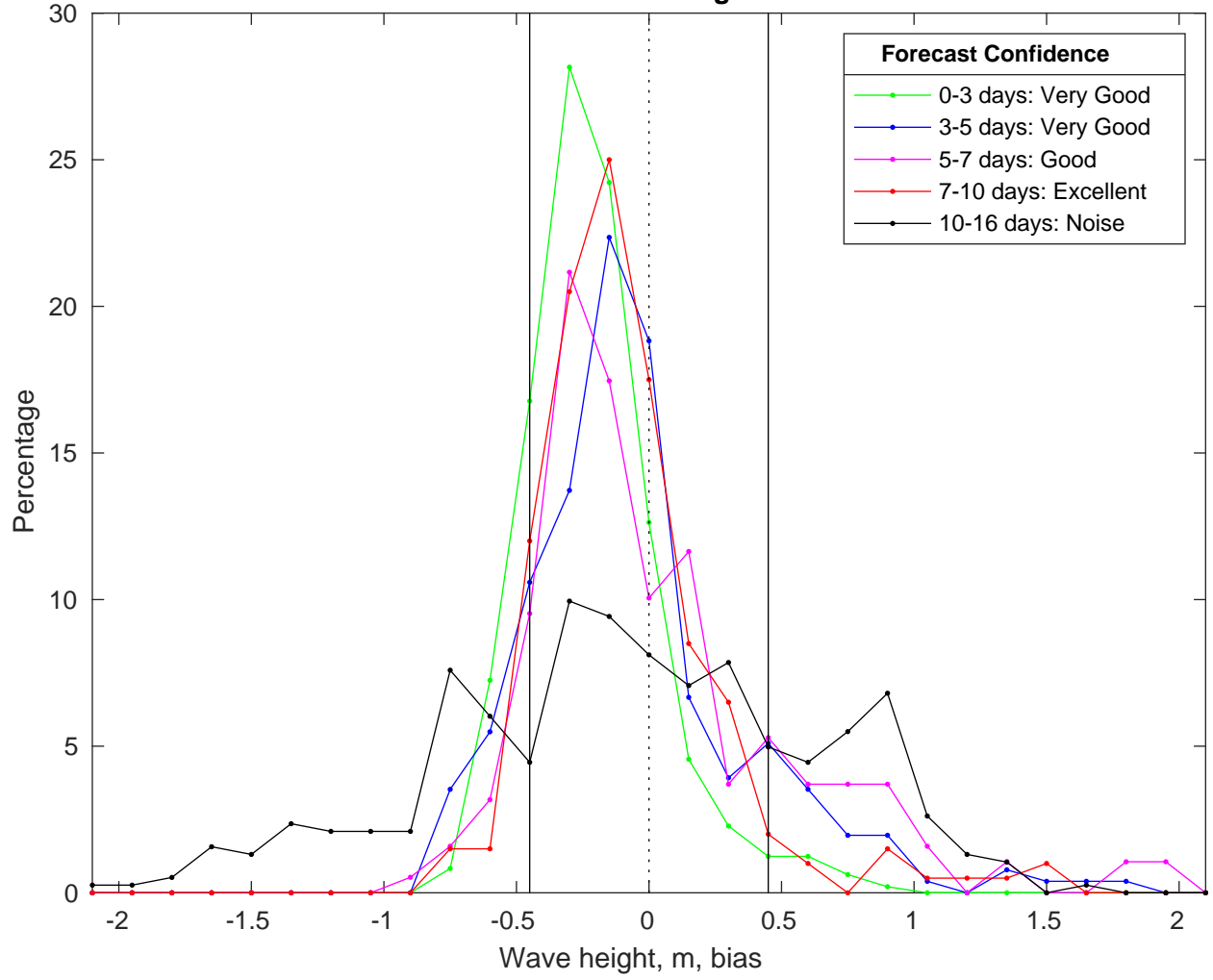
NDBC 46011 vs GFS Waves Bias Histogram: 08-Feb-2025
