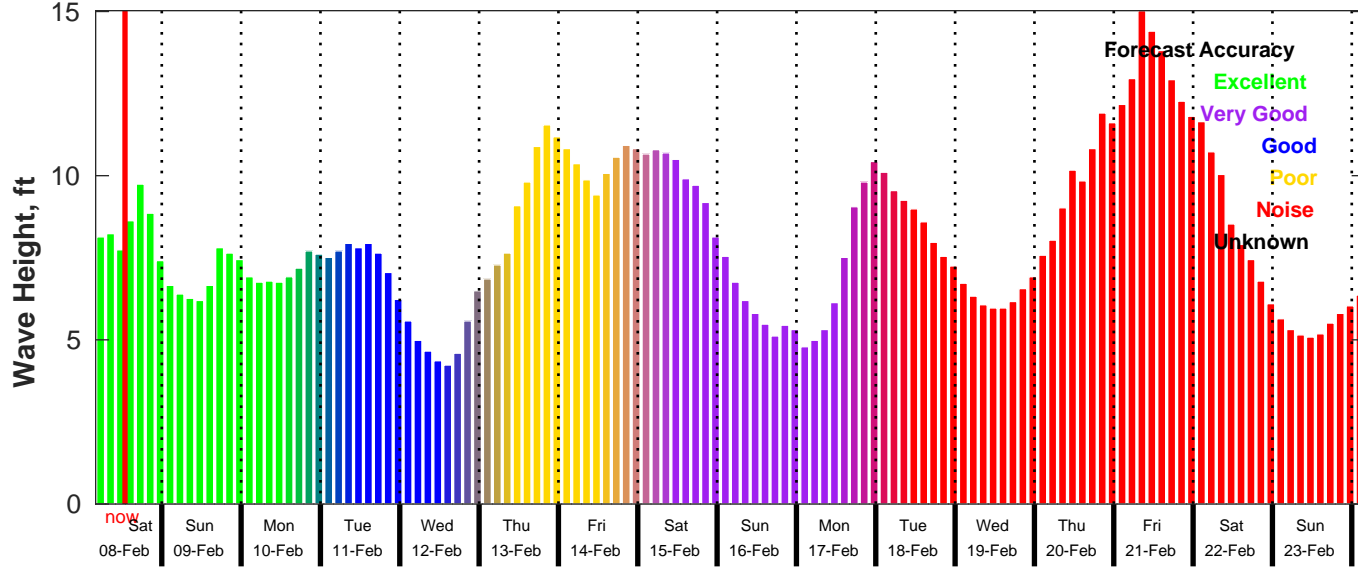
GFS Wave Forecast for NDBC 46028 from 08-Feb-2025 04:00:00 to 24-Feb-2025 04:00:00
