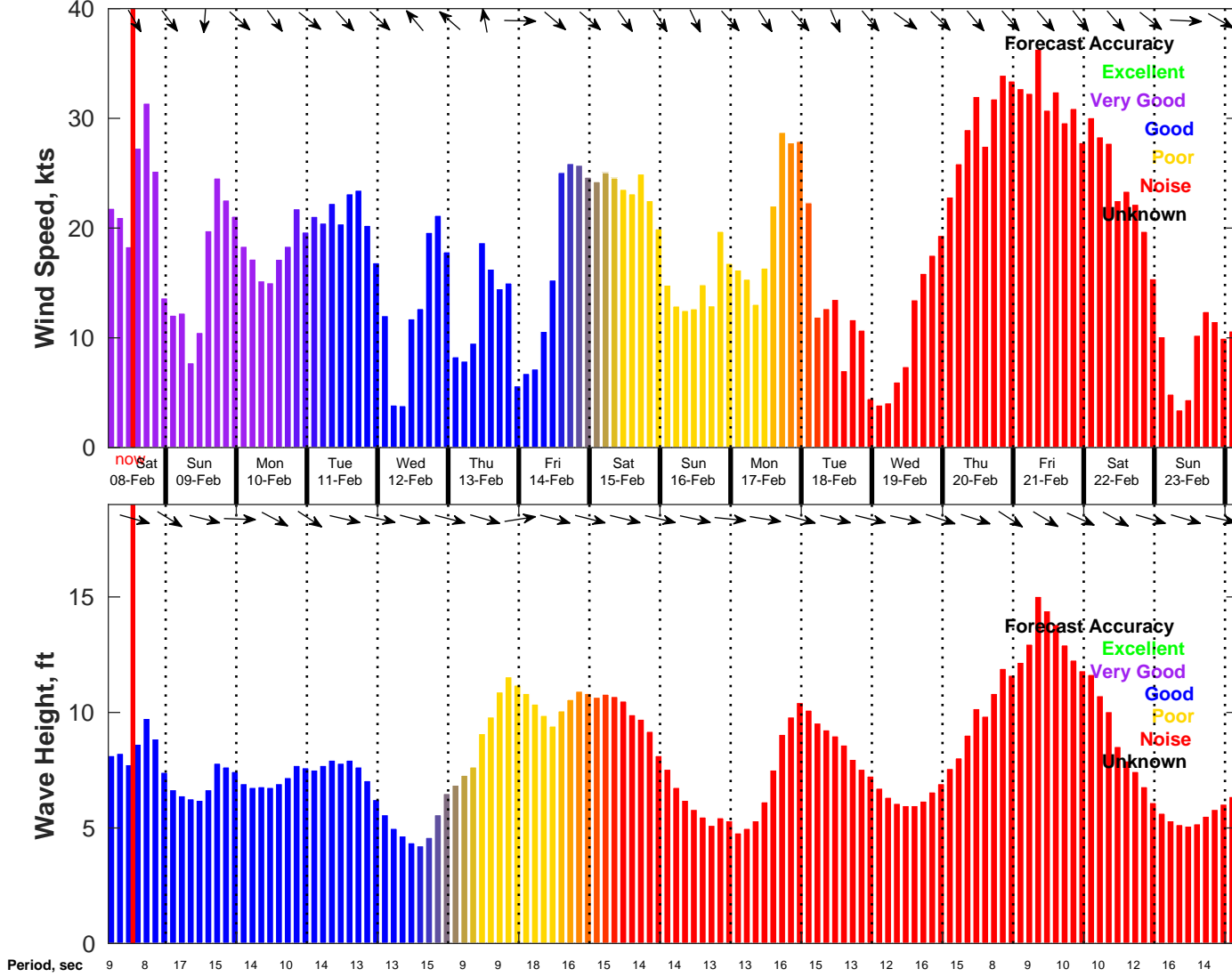
Wind & Wave Forecast for NDBC 46028 from 08-Feb-2025 04:00:00 to 24-Feb-2025 04:00:00
