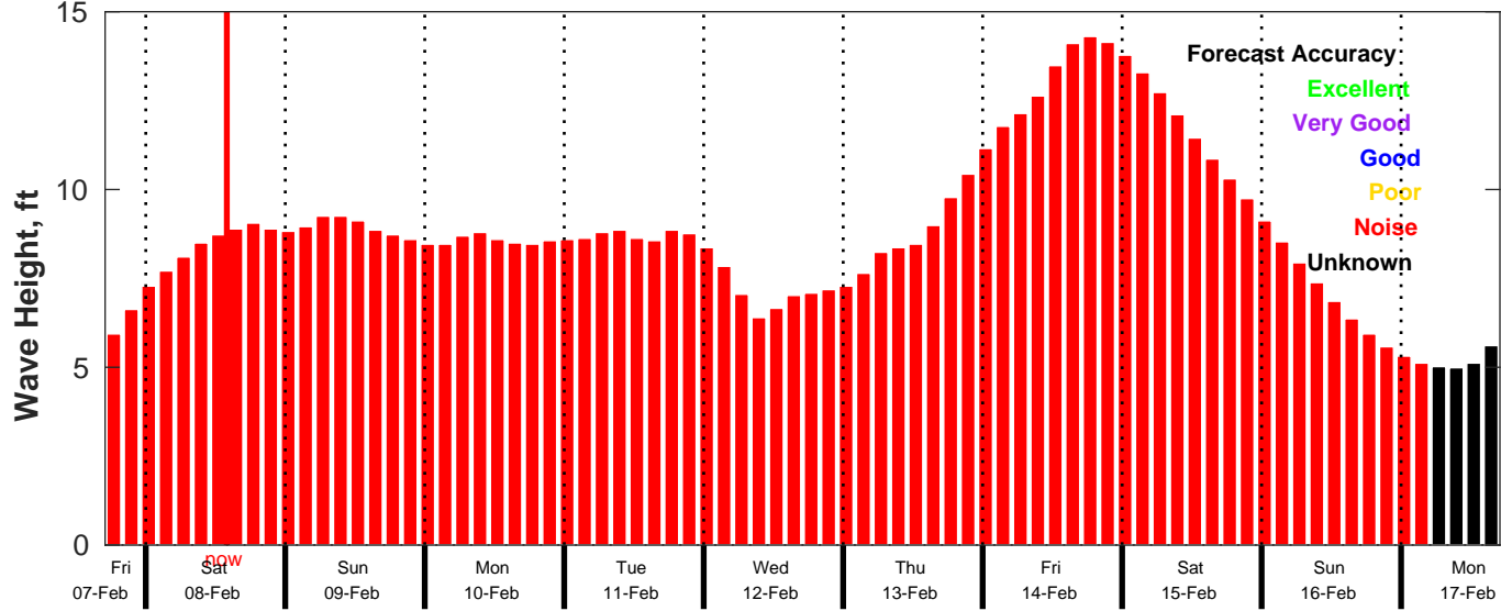
CMEMS Wave Forecast for NDBC 46053 from 07-Feb-2025 17:00:00 to 17-Feb-2025 17:00:00
