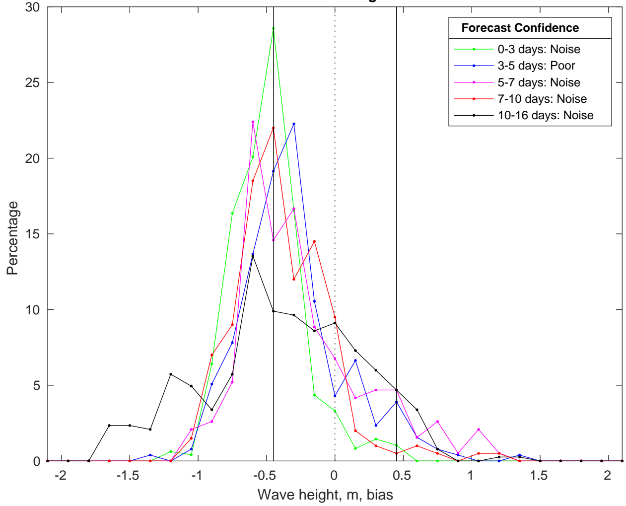
NDBC 46054 vs GFS Waves Bias Histogram: 08-Feb-2025
