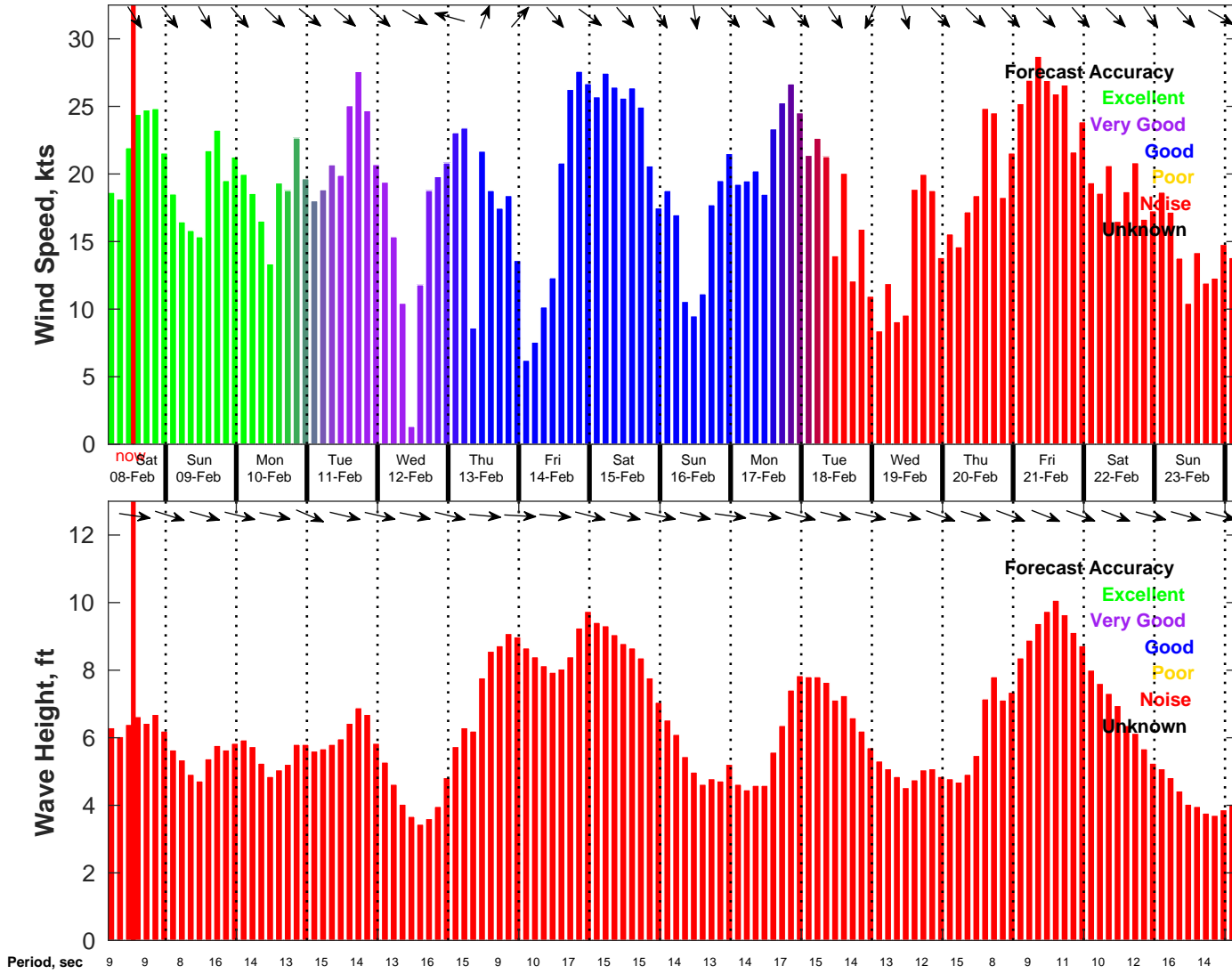
Wind & Wave Forecast for NDBC 46054 from 08-Feb-2025 04:00:00 to 24-Feb-2025 04:00:00
