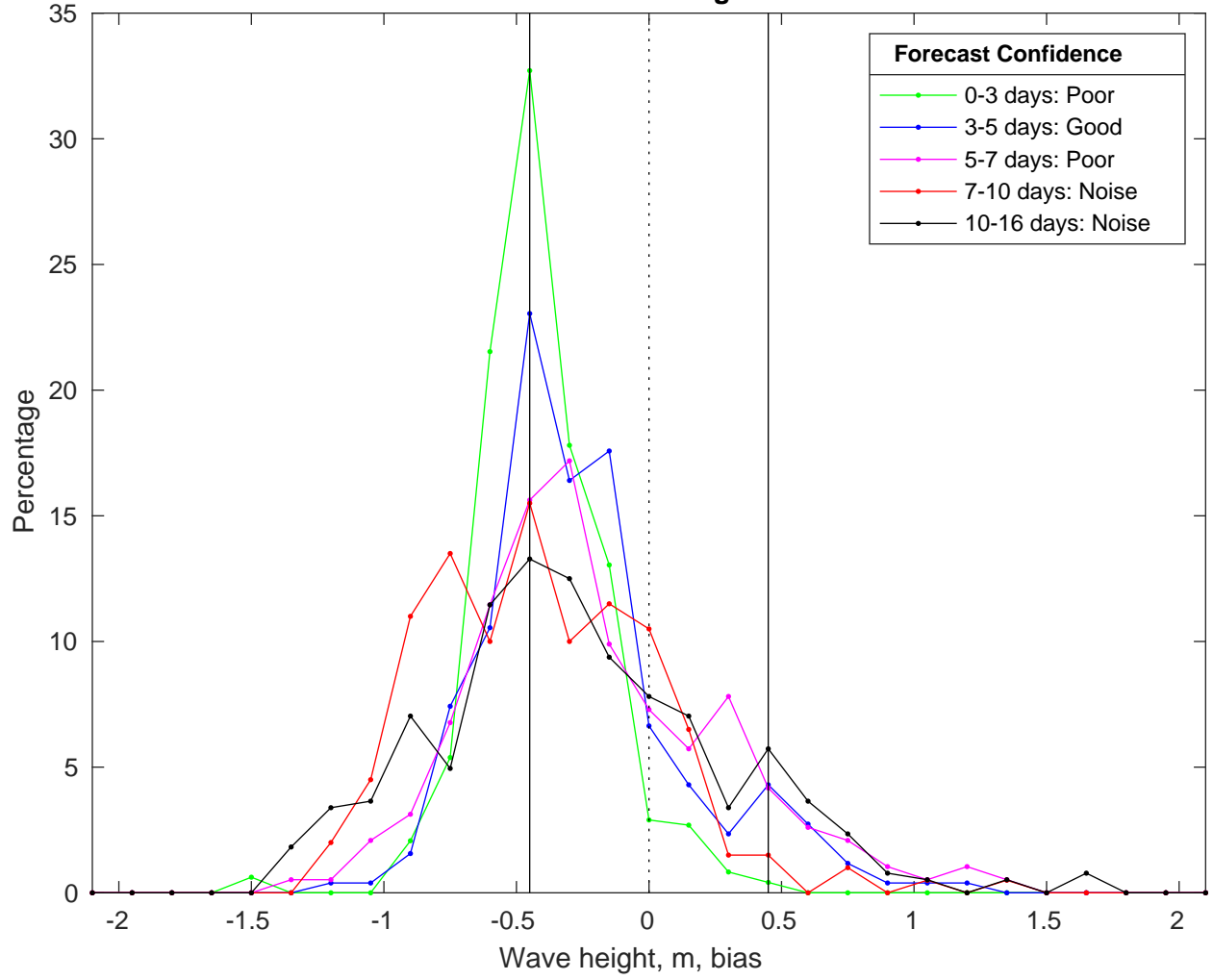
NDBC 46069 vs GFS Waves Bias Histogram: 08-Feb-2025
