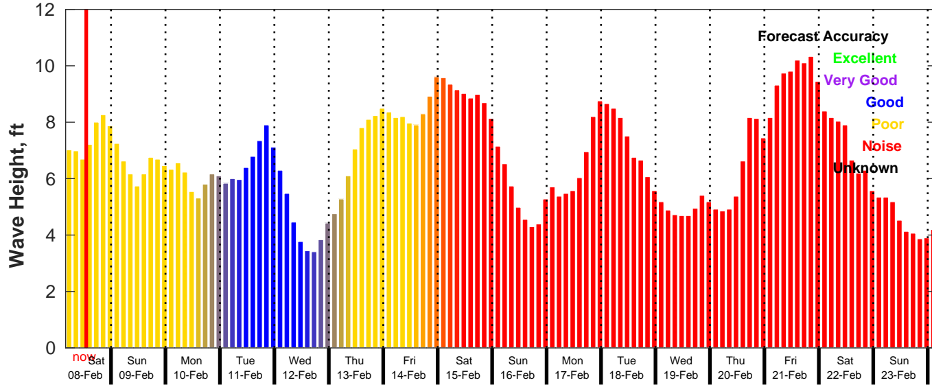
GFS Wave Forecast for NDBC 46069 from 08-Feb-2025 04:00:00 to 24-Feb-2025 04:00:00
