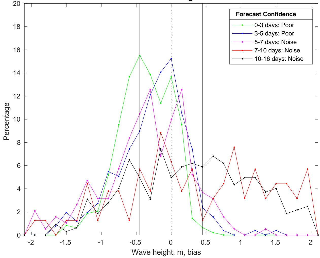
NDBC 46246 vs GFS Waves Bias Histogram: 08-Feb-2025
