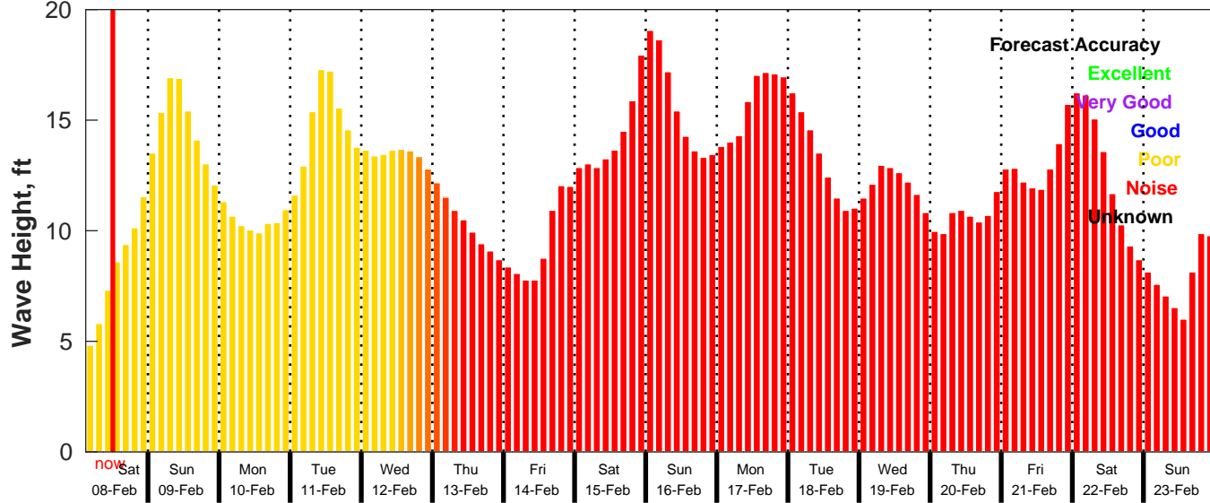
GFS Wave Forecast for NDBC 46246 from 08-Feb-2025 03:00:00 to 24-Feb-2025 03:00:00
