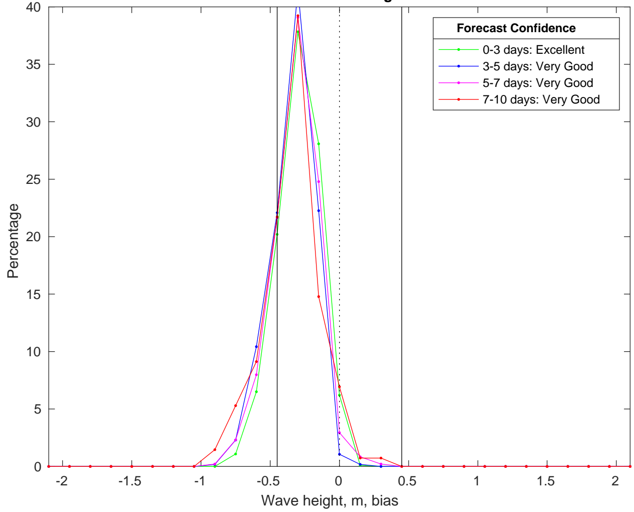
NDBC 51209 vs CMEMS Waves Bias Histogram: 08-Feb-2025
