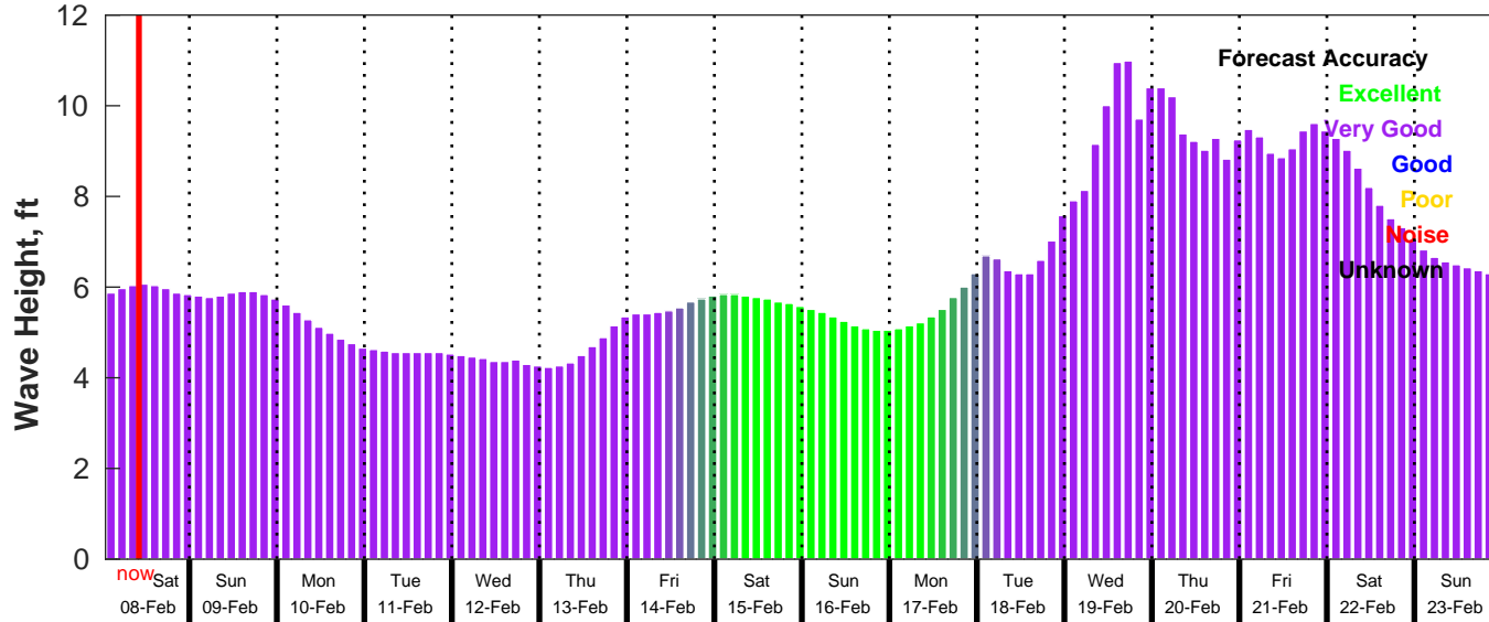
GFS Wave Forecast for NDBC 51209 from 08-Feb-2025 01:00:00 to 24-Feb-2025 01:00:00
