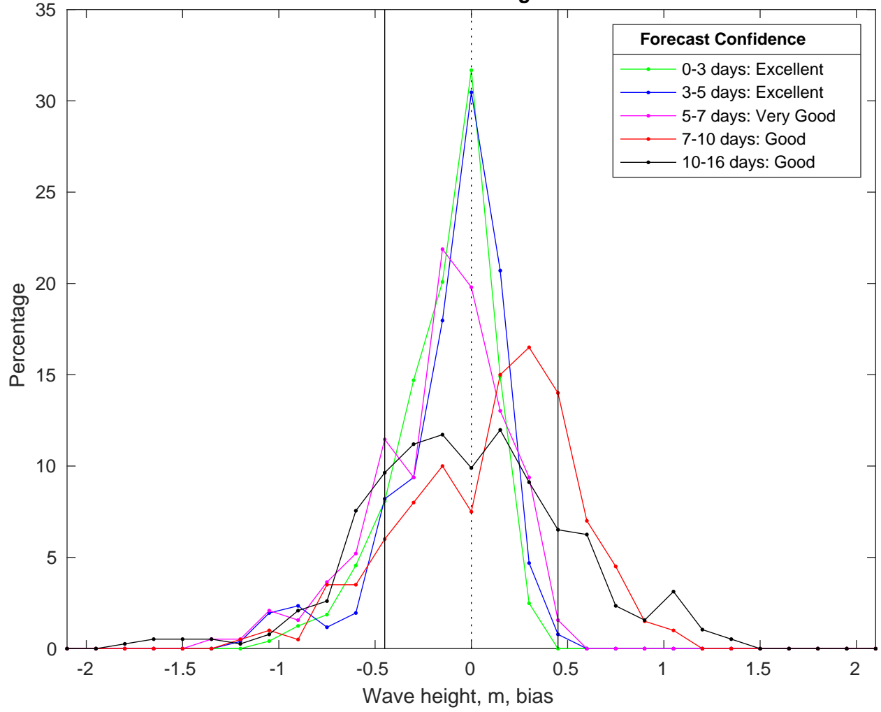
NDBC 52211 vs GFS Waves Bias Histogram: 08-Feb-2025
