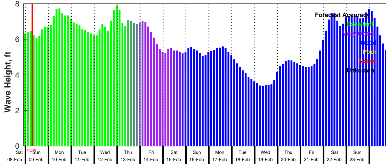
GFS Wave Forecast for NDBC 52211 from 08-Feb-2025 22:00:00 to 24-Feb-2025 22:00:00
