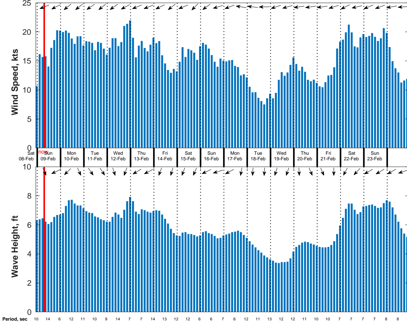
Wind & Wave Forecast for NDBC 52211 from 08-Feb-2025 22:00:00 to 24-Feb-2025 22:00:00
