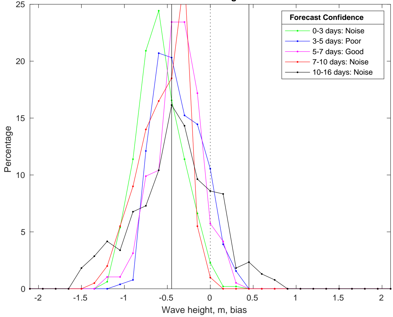
NDBC 52213 vs GFS Waves Bias Histogram: 08-Feb-2025
