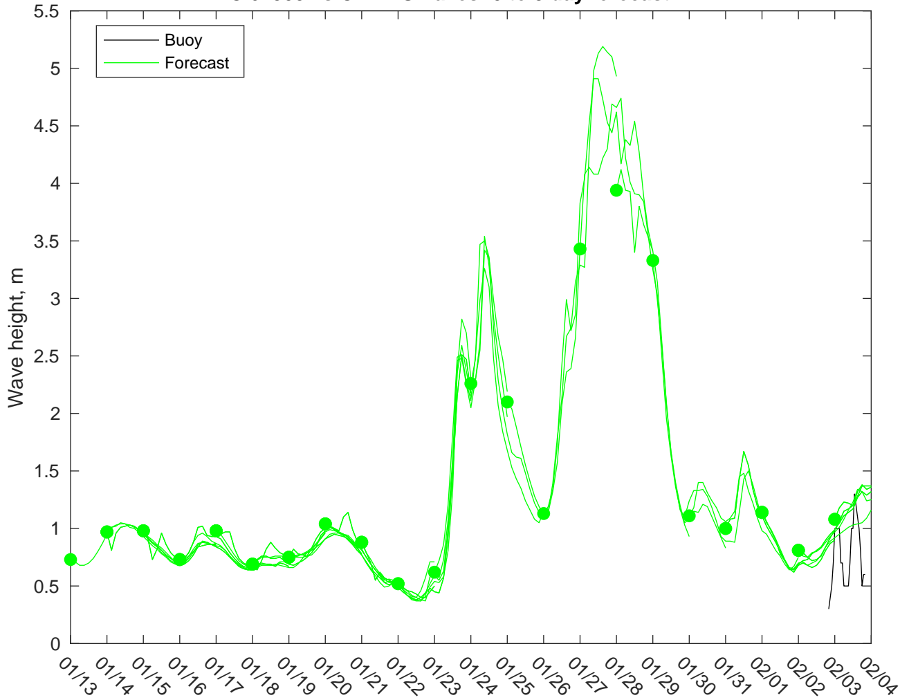
NDBC 62305 vs CMEMSWaves: 0 to 3 day forecast
