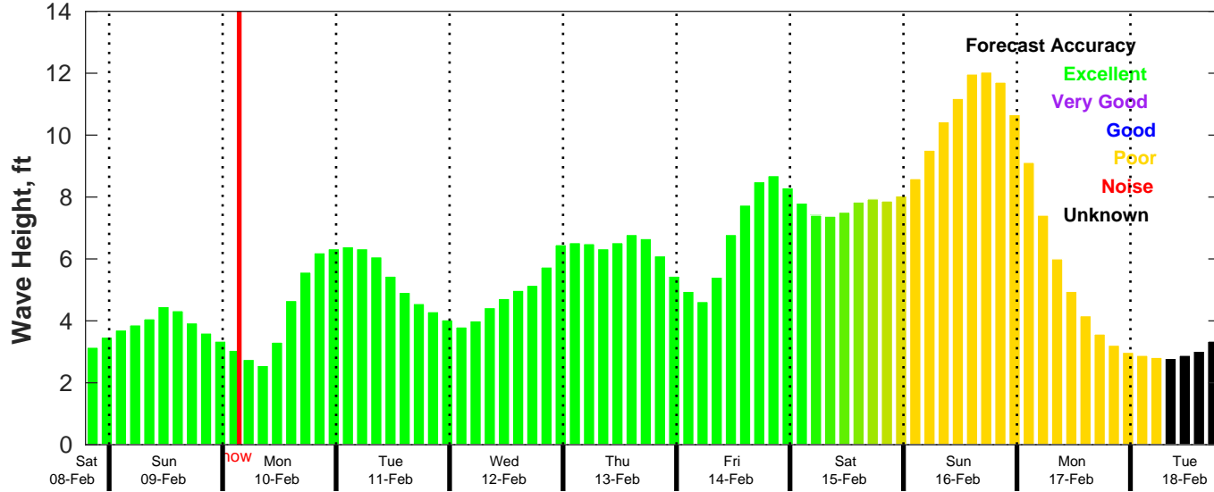
CMEMS Wave Forecast for NDBC 41004 from 08-Feb-2025 19:00:00 to 18-Feb-2025 19:00:00
