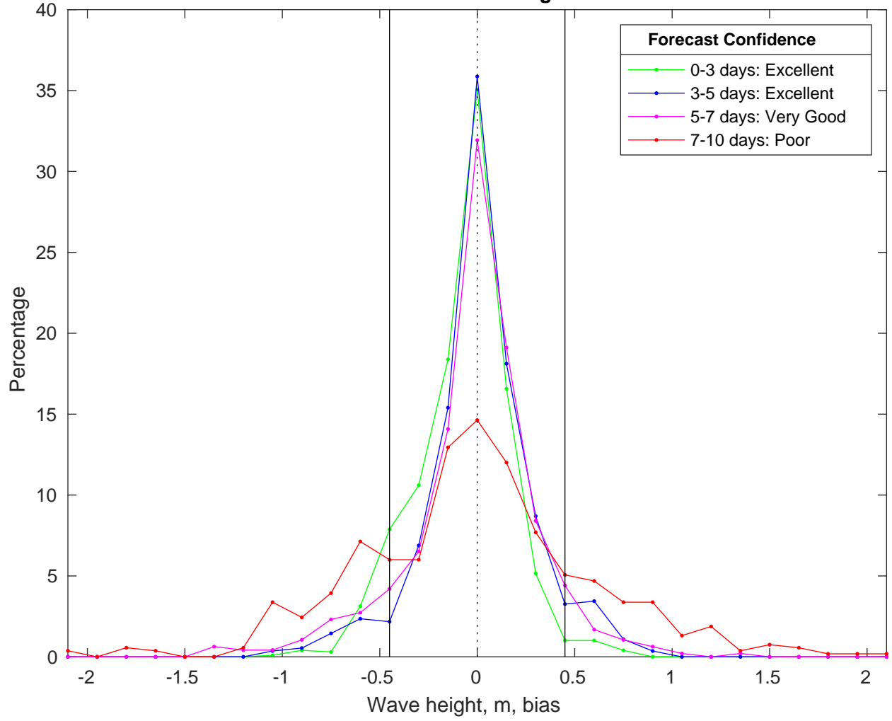
NDBC 41013 vs CMEMS Waves Bias Histogram: 09-Feb-2025
