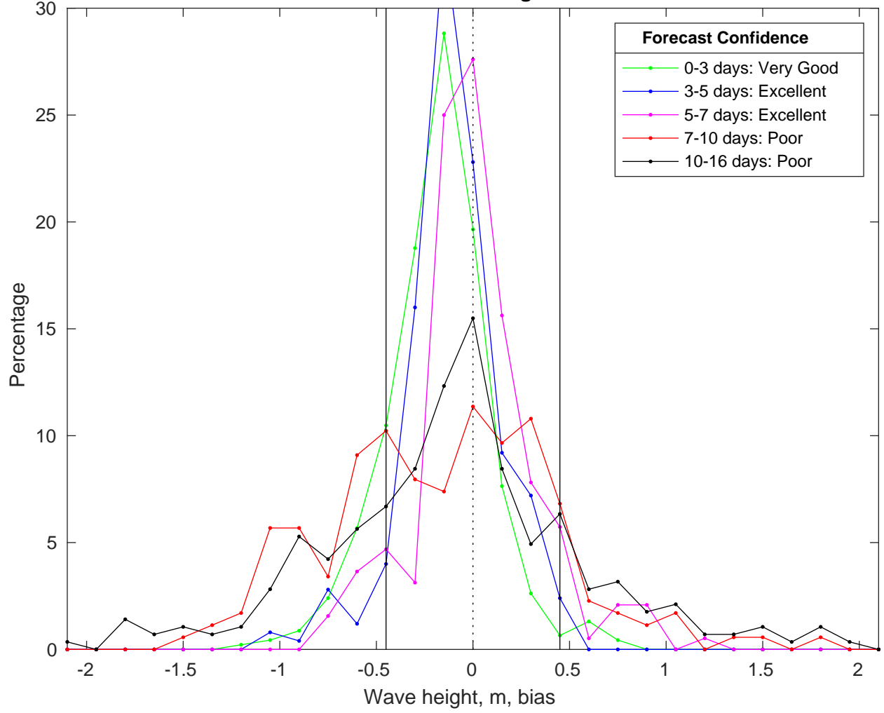
NDBC 41013 vs GFS Waves Bias Histogram: 09-Feb-2025
