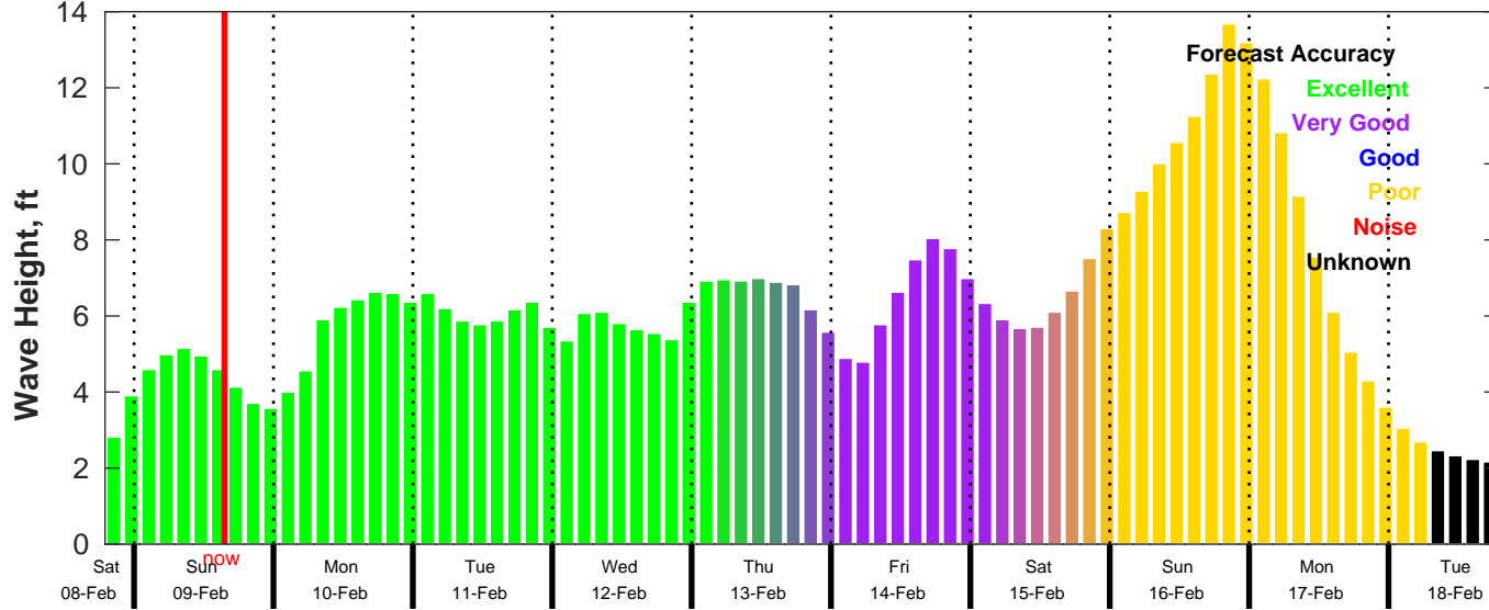
CMEMS Wave Forecast for NDBC 41013 from 08-Feb-2025 19:00:00 to 18-Feb-2025 19:00:00
