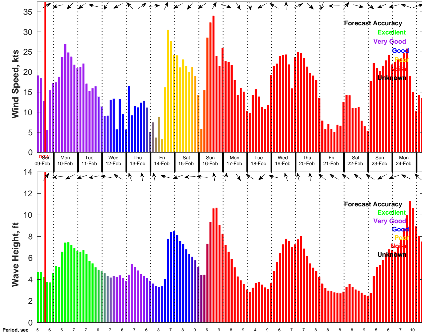
Wind & Wave Forecast for NDBC 41013 from 09-Feb-2025 07:00:00 to 25-Feb-2025 07:00:00
