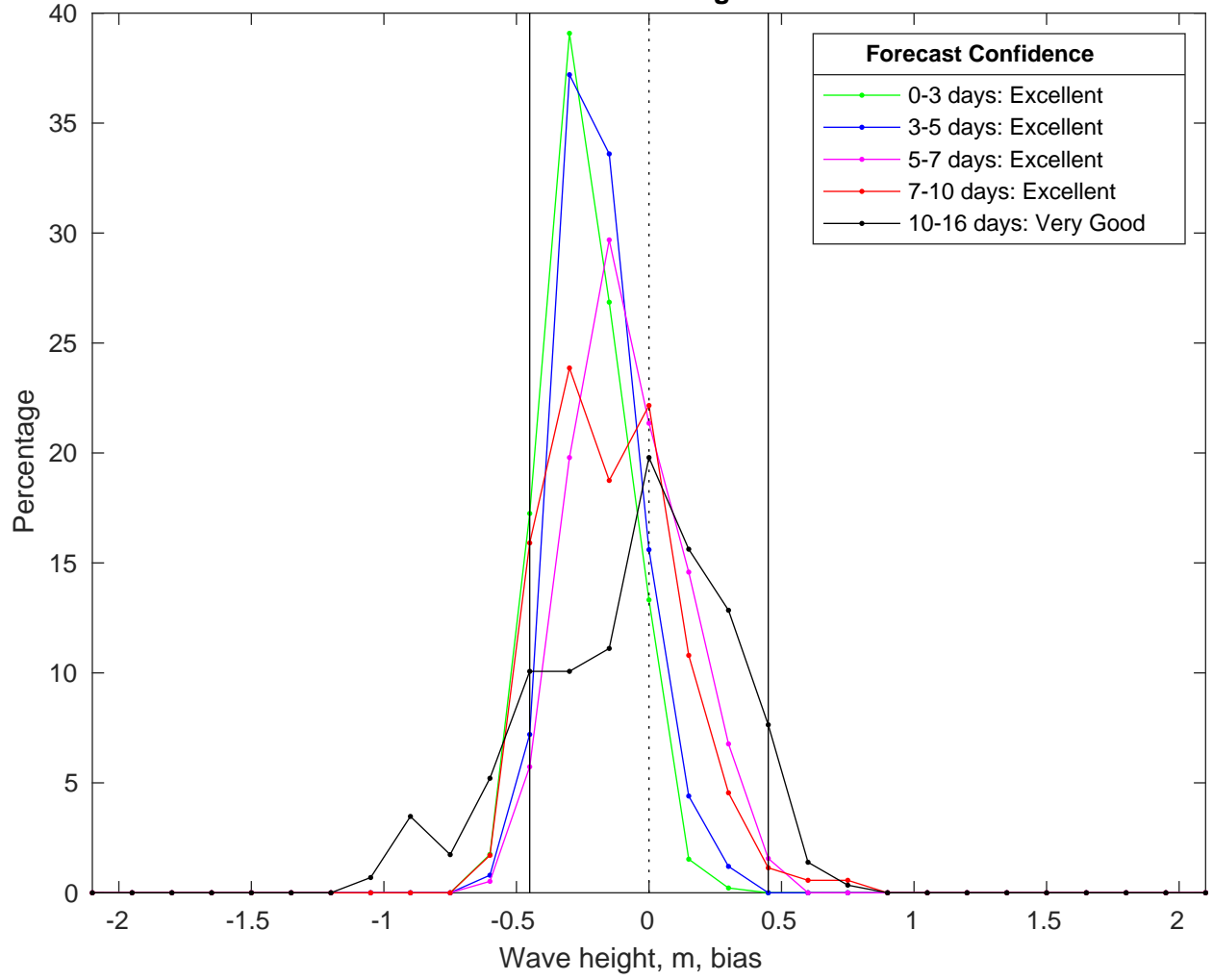
NDBC 41040 vs GFS Waves Bias Histogram: 09-Feb-2025
