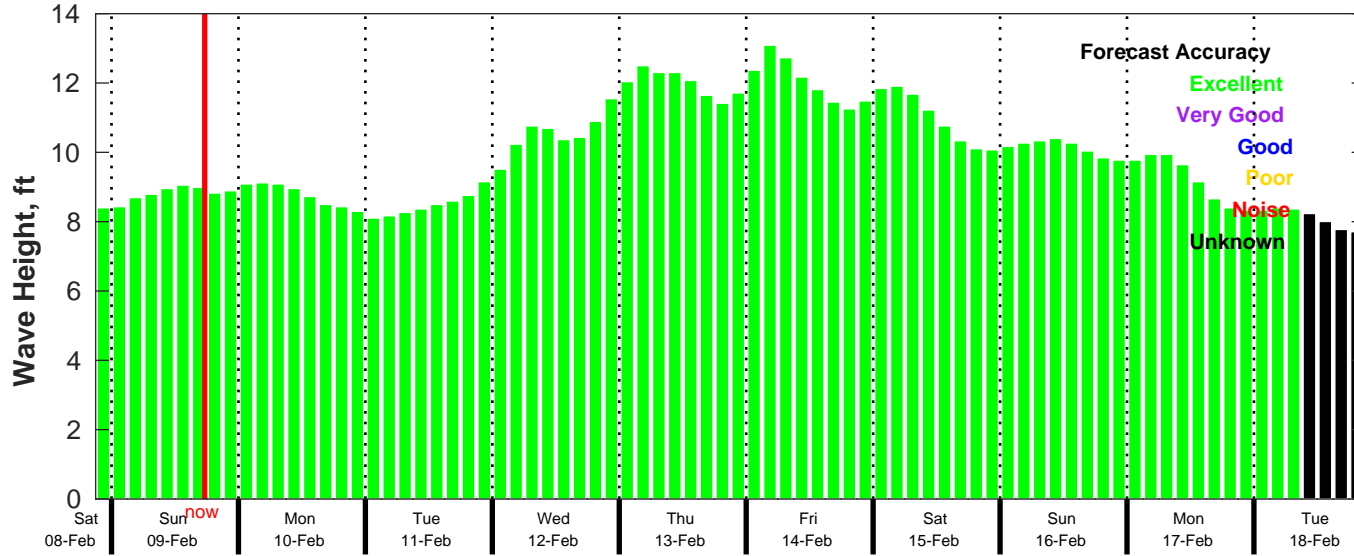
CMEMS Wave Forecast for NDBC 41040 from 08-Feb-2025 21:00:00 to 18-Feb-2025 21:00:00
