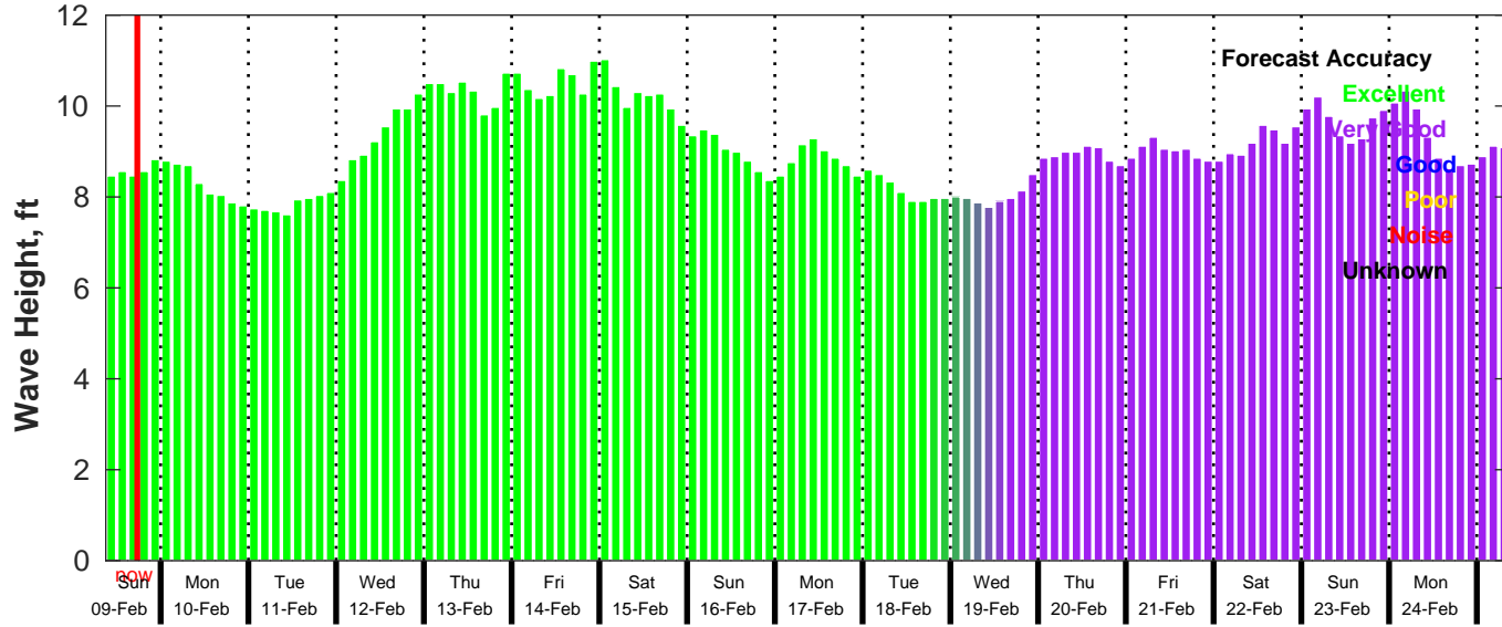
GFS Wave Forecast for NDBC 41040 from 09-Feb-2025 09:00:00 to 25-Feb-2025 09:00:00
