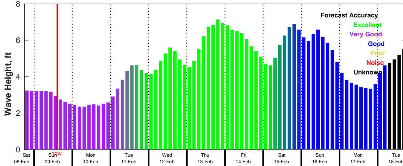
CMEMS Wave Forecast for NDBC 42019 from 08-Feb-2025 18:00:00 to 18-Feb-2025 18:00:00
