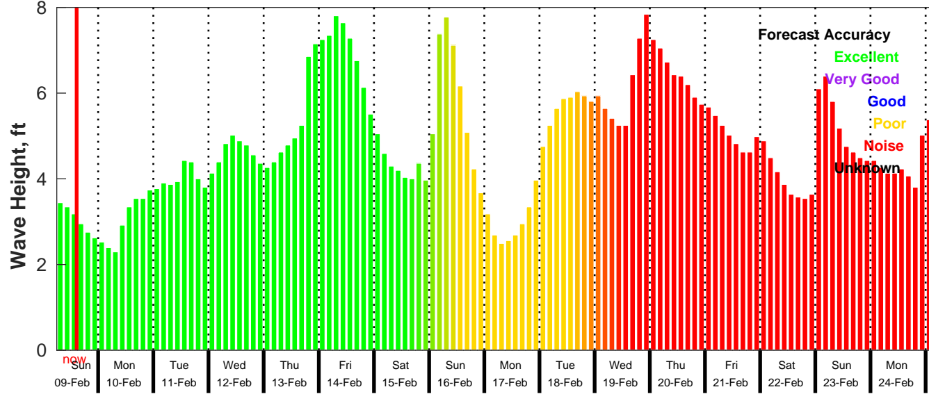
GFS Wave Forecast for NDBC 42019 from 09-Feb-2025 06:00:00 to 25-Feb-2025 06:00:00
