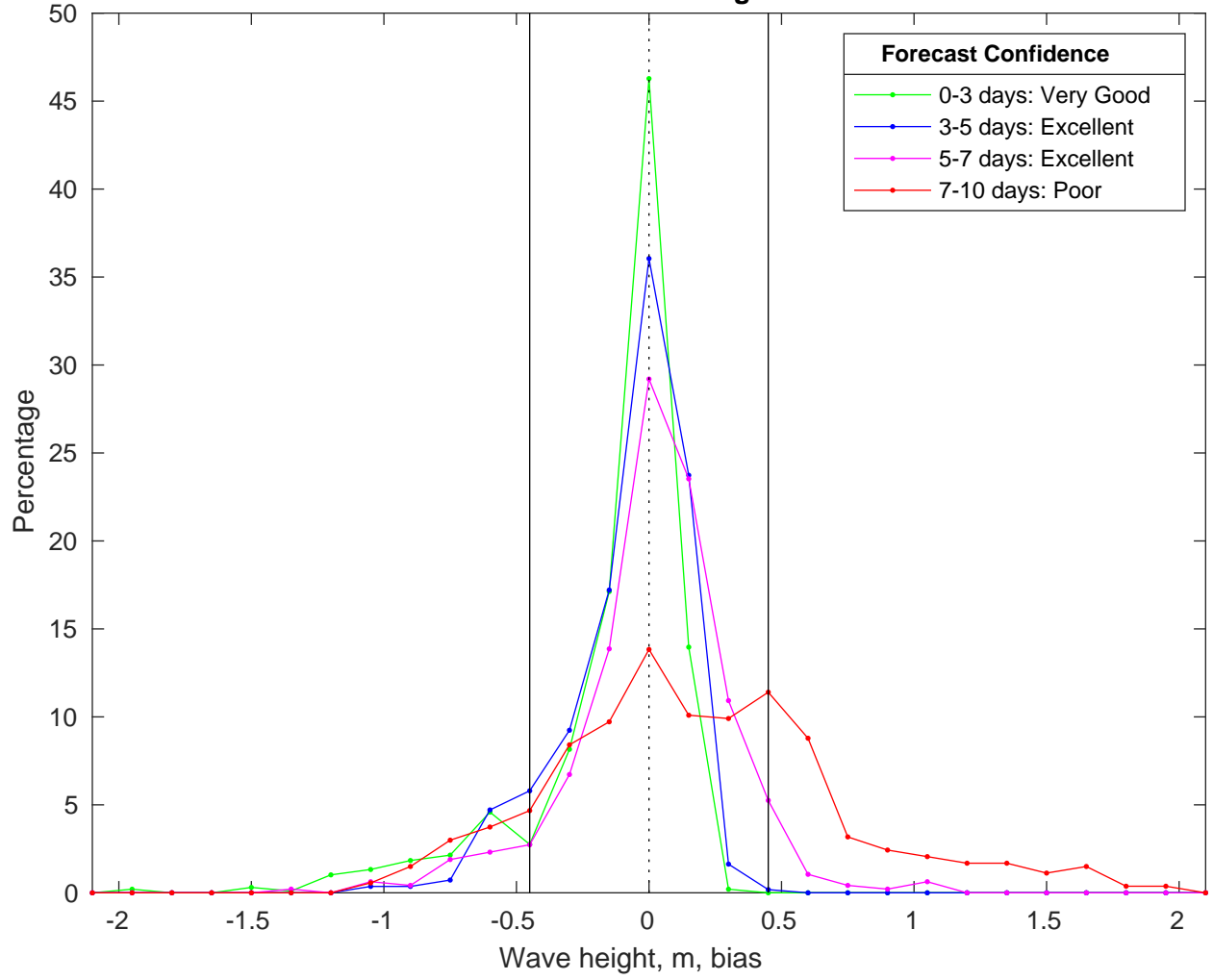
NDBC 42020 vs CMEMS Waves Bias Histogram: 09-Feb-2025
