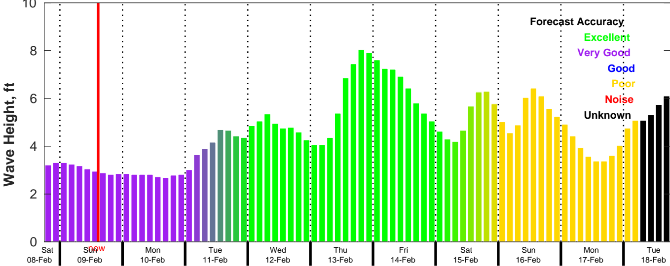
CMEMS Wave Forecast for NDBC 42020 from 08-Feb-2025 18:00:00 to 18-Feb-2025 18:00:00
