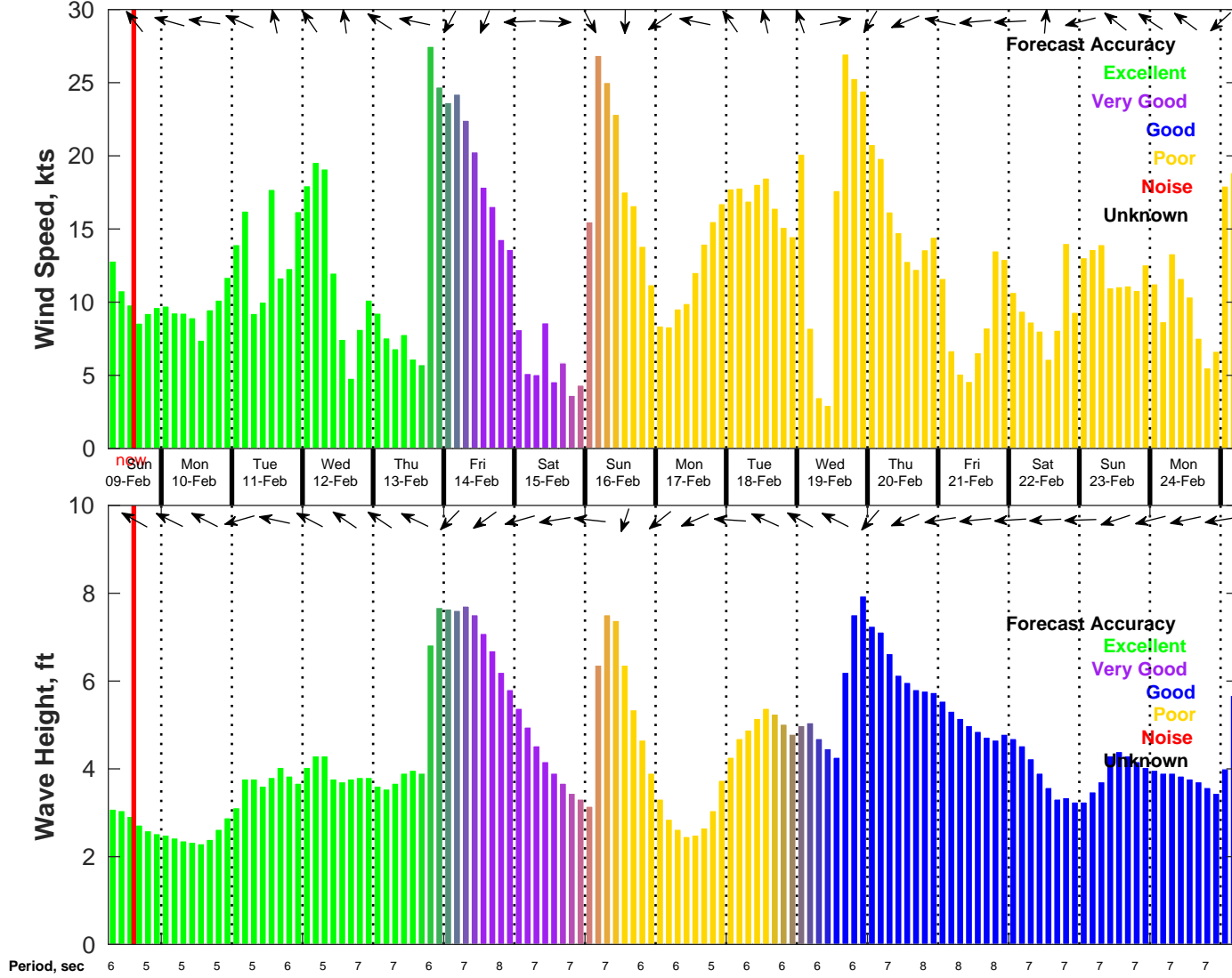
Wind & Wave Forecast for NDBC 42020 from 09-Feb-2025 06:00:00 to 25-Feb-2025 06:00:00
