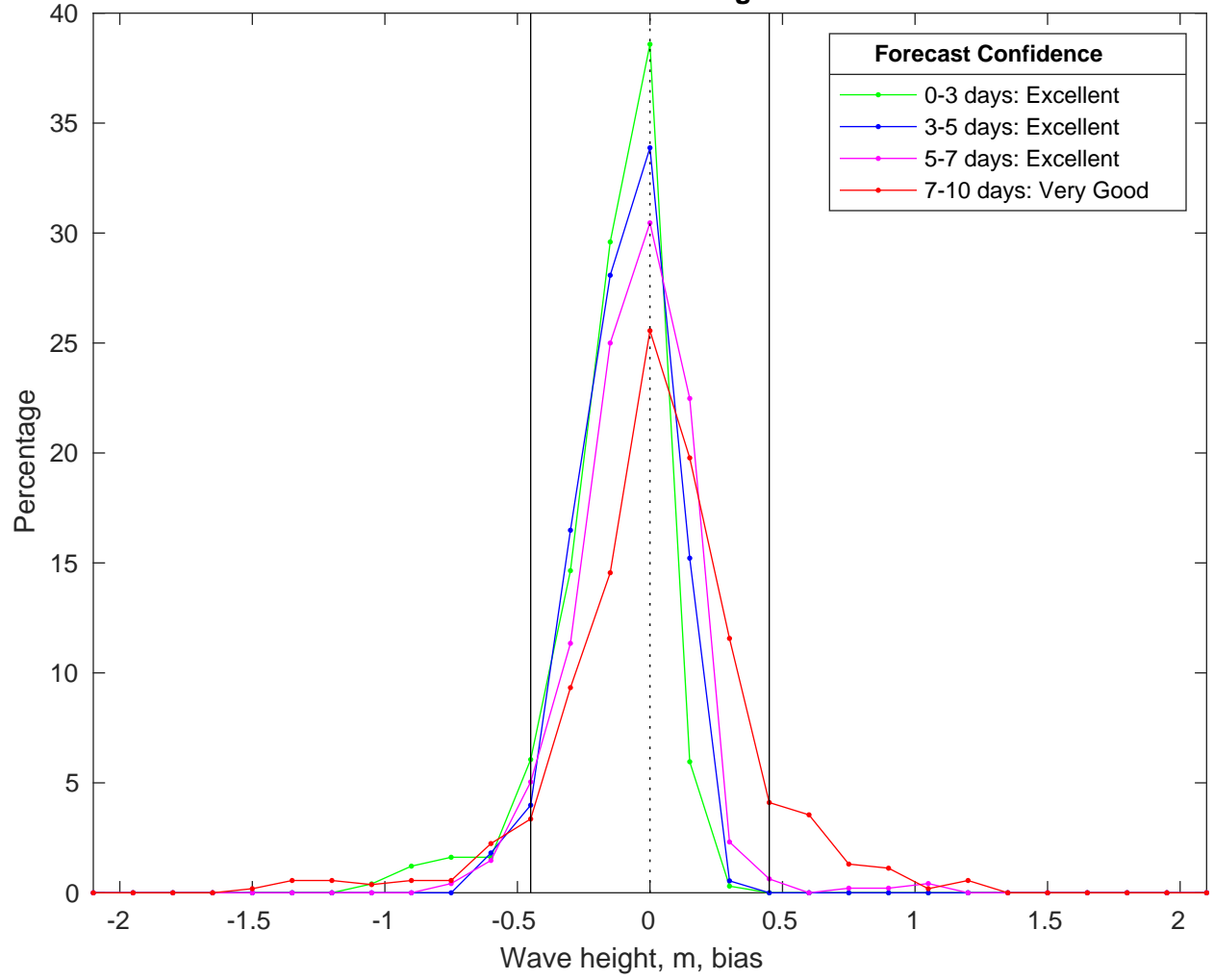
NDBC 42035 vs CMEMS Waves Bias Histogram: 09-Feb-2025
