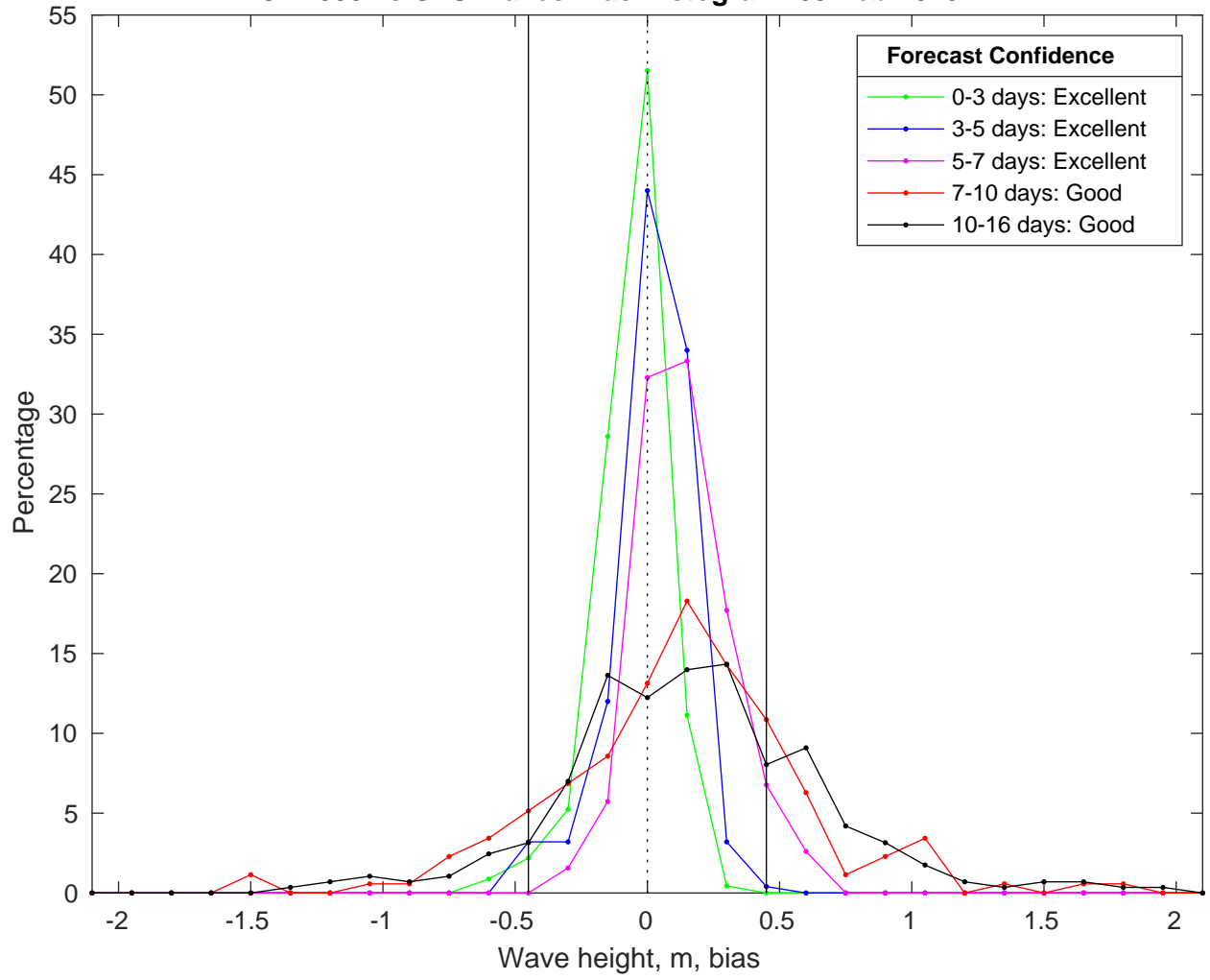
NDBC 42035 vs GFS Waves Bias Histogram: 09-Feb-2025
