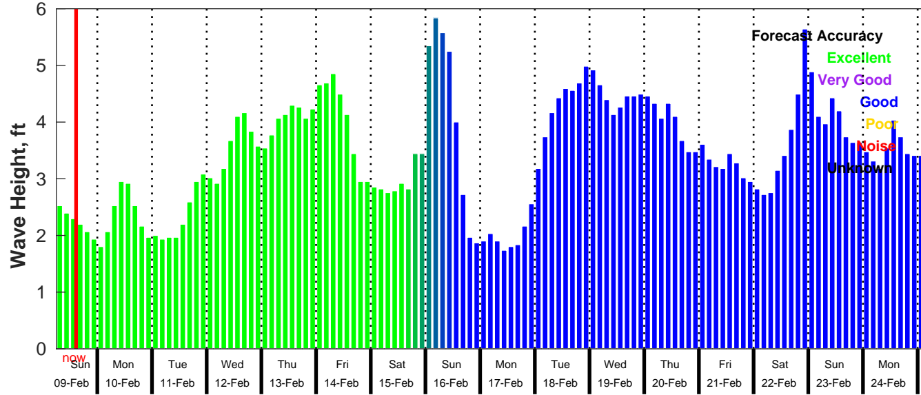
GFS Wave Forecast for NDBC 42035 from 09-Feb-2025 06:00:00 to 25-Feb-2025 06:00:00
