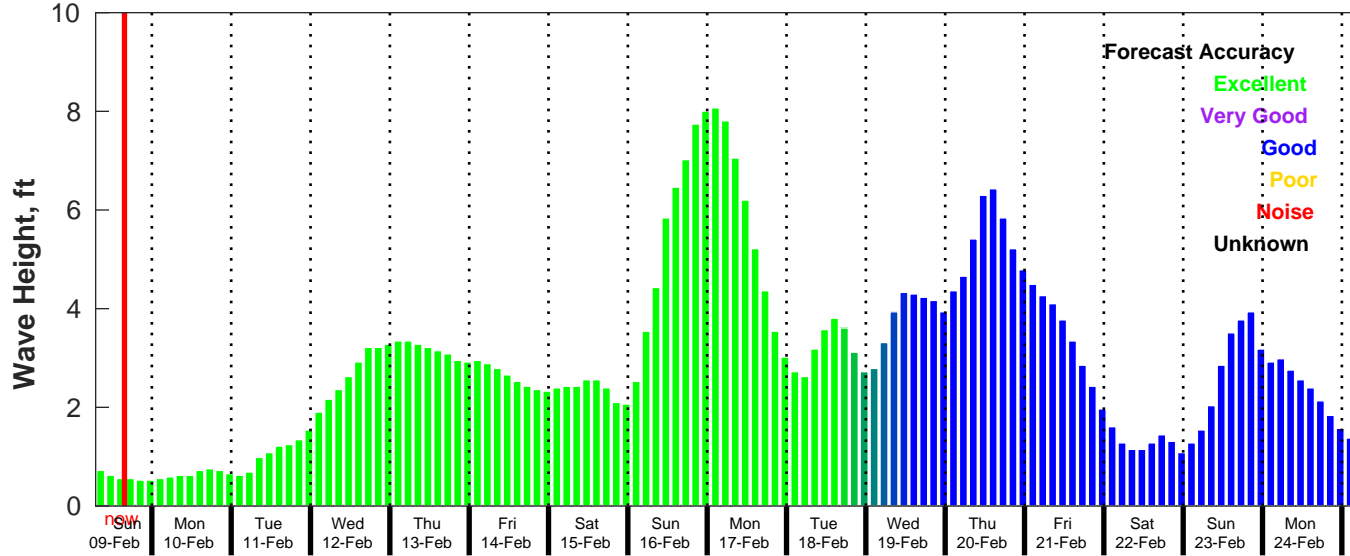
GFS Wave Forecast for NDBC 42036 from 09-Feb-2025 07:00:00 to 25-Feb-2025 07:00:00
