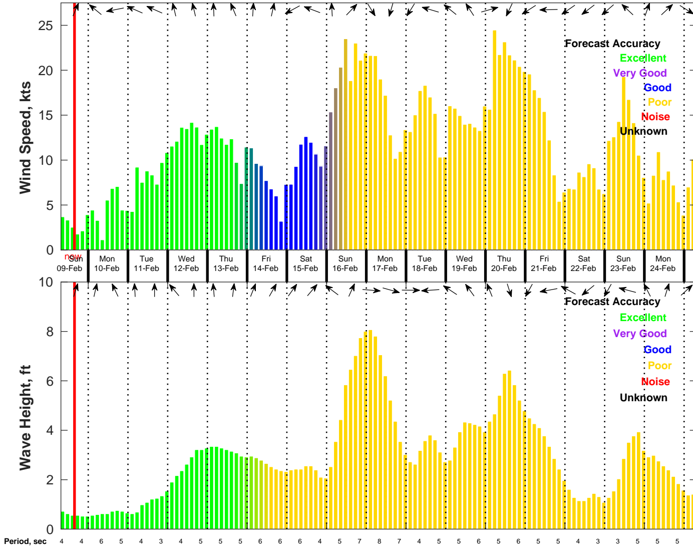
Wind & Wave Forecast for NDBC 42036 from 09-Feb-2025 07:00:00 to 25-Feb-2025 07:00:00
