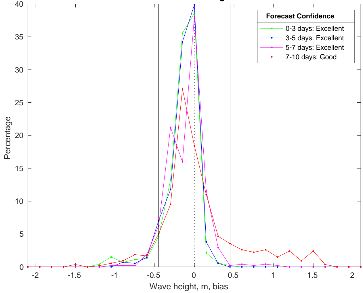
NDBC 42040 vs CMEMS Waves Bias Histogram: 09-Feb-2025
