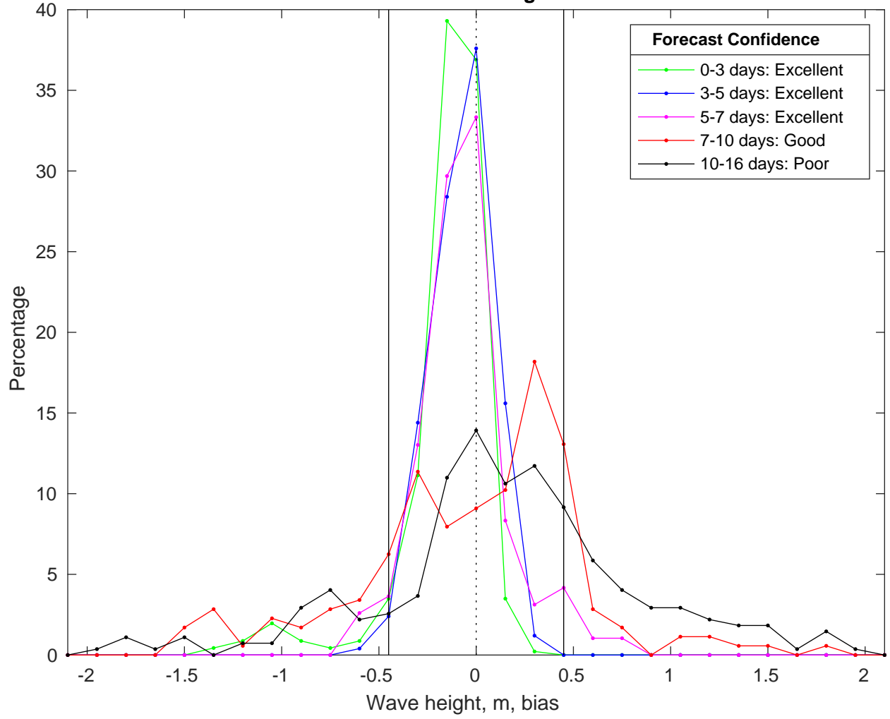
NDBC 42040 vs GFS Waves Bias Histogram: 09-Feb-2025
